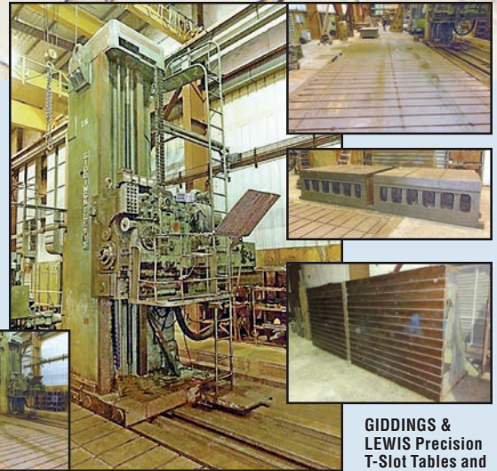
GIDDINGS & LEWIS 570 Faur Horizontal Boring Mill , 7" spindle, #7 Morse taper, X=432", Y=192", Z=156" vertical, 44" runway, w/Trak i02 2-axis DRO, SN 280-1455.
